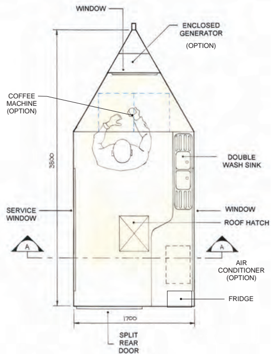
PLAN VIEW: COFFEE CART
